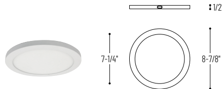
NLOCAC-8R345W 8" CAMO
