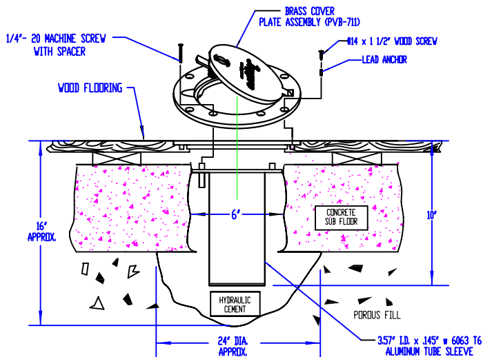
TYPICAL INSTALLATION IN A FINISHED WOOD FLOOR
