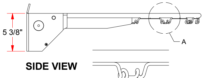
PIG TAIL NET ATTACHMENT SYSTEM (12 PLACES)
