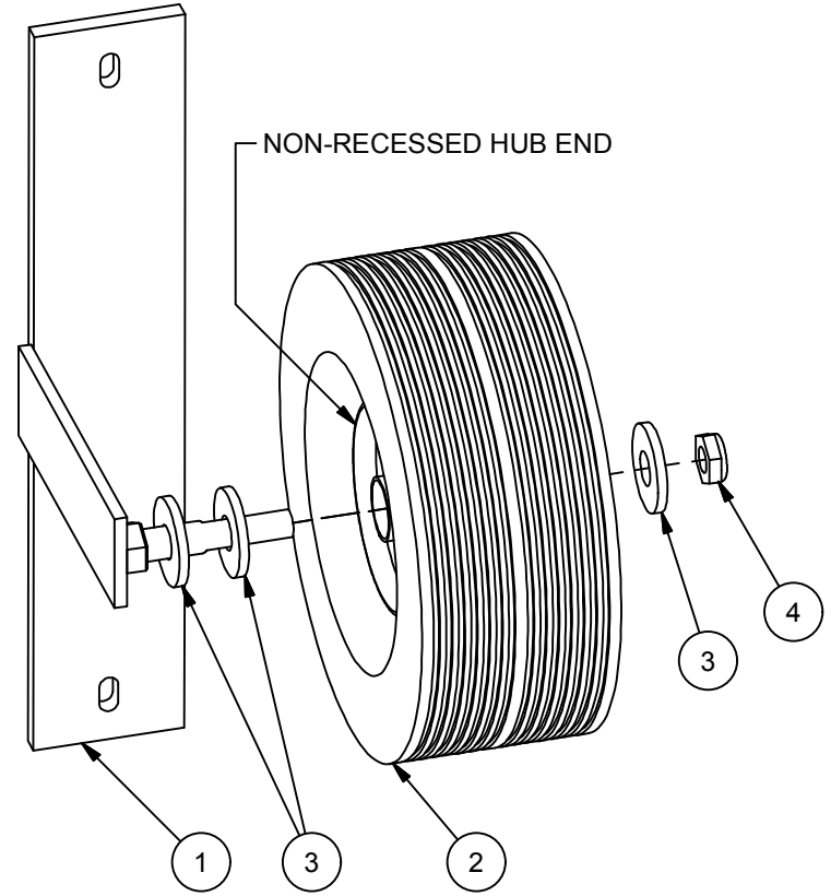
EXPLODED VIEW
