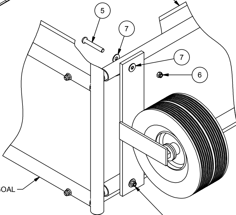
DETAIL A (SEE EXPLODED VIEW)
