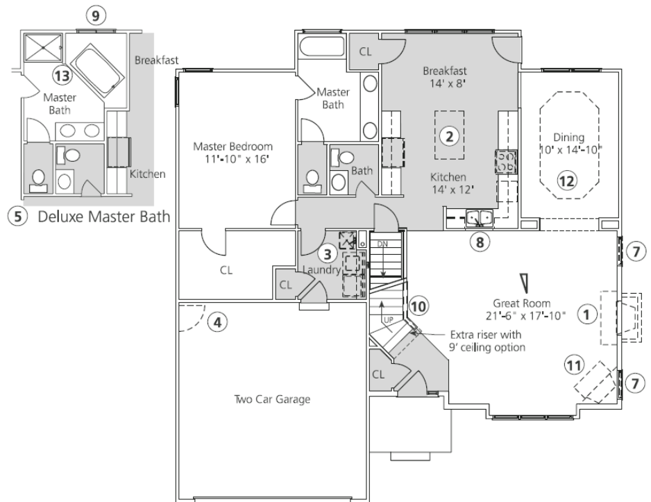
First Floor (Elevation "A")
