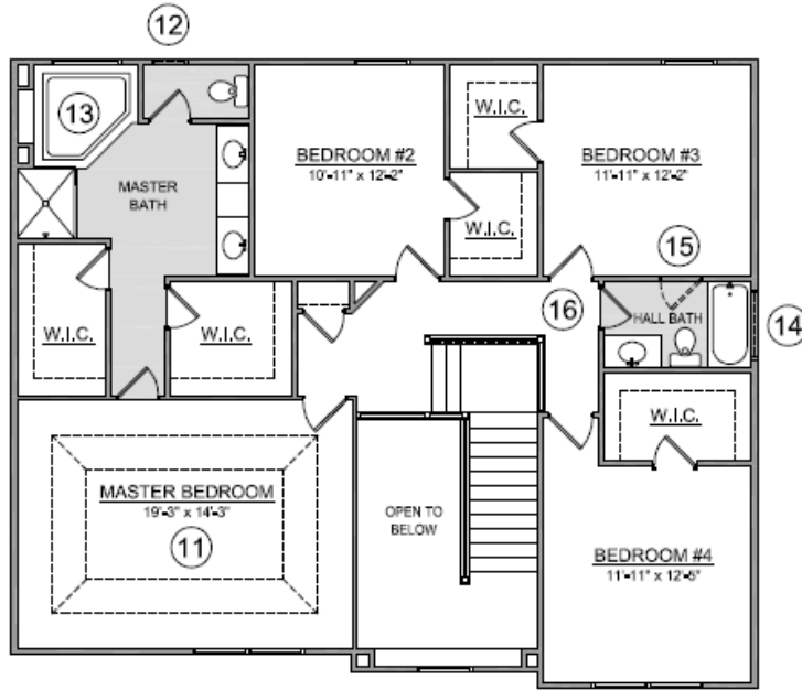
Second Floor (Elevation "A")
